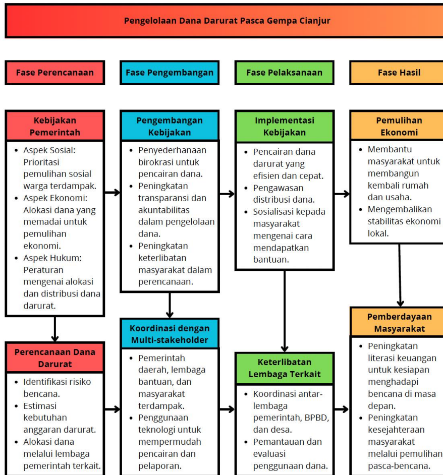
Gambar 1. Research Framework
